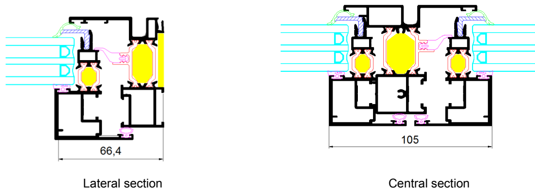
Figure 1: Representative scheme of System AJi- Hidden Leaf Channel 16 by Anicolor (dimensions in mm).
