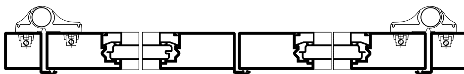
Section B-B
