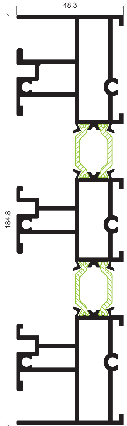
CTe-11 Padieira tri-rail Marco superior tricarril
