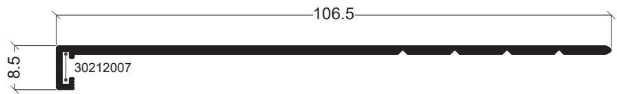
S-22 Remate Solape 106.5x8.5mm
