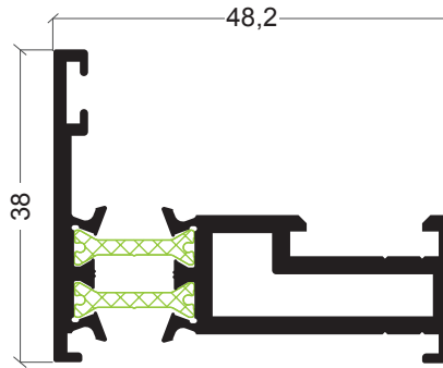
CW-24 Prumo Central CW minimal Prumo Central CW minimal
